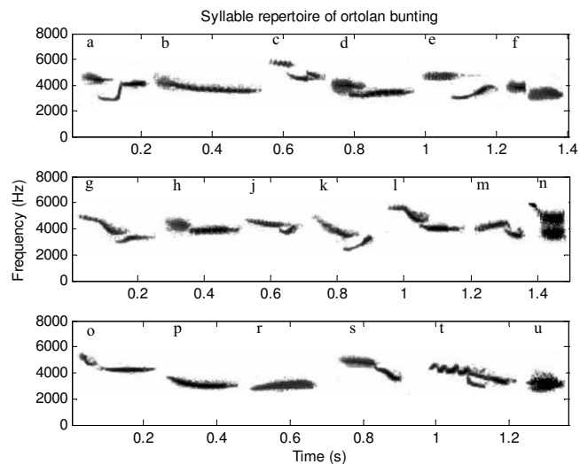
FIG. 1. Complete set of the 19-syllable repertoire of ortolan bunting.
