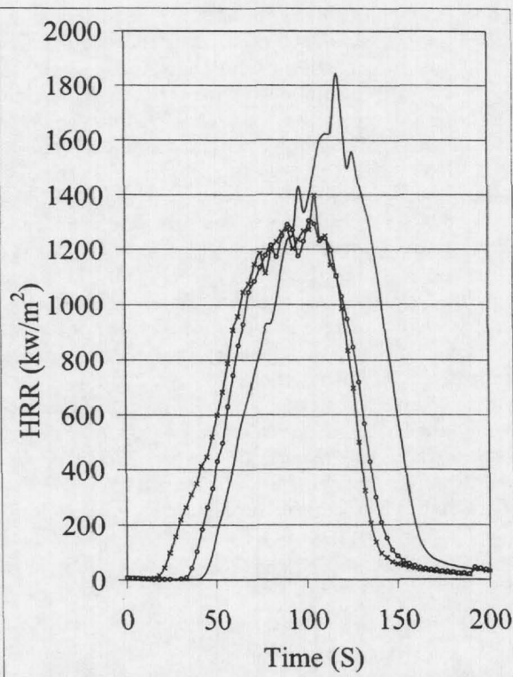
Figure 7. The heat release rate curves for polystyrene,—, the potassium dicyclohexano-18-crown-6 nanocomposite, X, and the potassium dibenzo-18-crown-6 nanocomposite, O.
