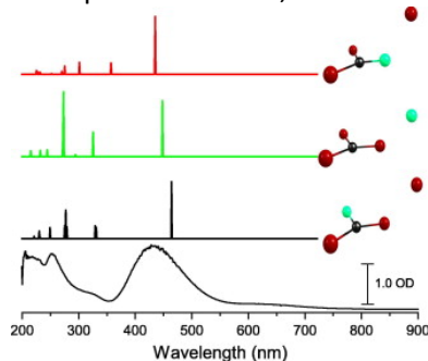
Fig. 4. UV–Vis spectrum following 220 nm laser photolysis of a CClBr 3 :Ar sample held at 5 K and calculated (TD M06/aug-cc-pVTZ) electronic spectra of the three possible iso-CClBr 3 isomers. The calculated spectra are shown as stick spectra and the intensities are arbitrarily scaled; quantitative information is provided in Table 2 .
