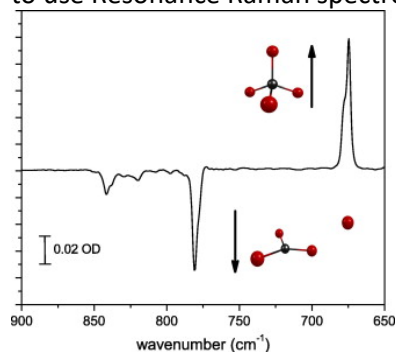
Fig. 9. Difference spectrum following 440 nm excitation of matrix-isolated iso- \text{CBr}_4 . Laser irradiation of the isomer leads to loss of the isomer IR bands and reformation of the parent halon.
