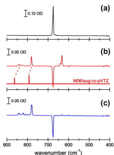
Fig. 5. (a) Infrared (IR) spectrum of a CBr 4 :Ar sample at 5 K. (b) Difference IR spectrum following photolysis of the sample at 266 nm. The calculated (M06/aug-cc-pVTZ) spectrum of iso-CBr 4 is shown as a stick spectrum in this panel, and the intensity is arbitrarily scaled; quantitative information is provided in Table 4 . (c) Difference IR spectrum following photolysis at 266 nm and subsequent annealing to 30 K, following by recooling to 5 K.
