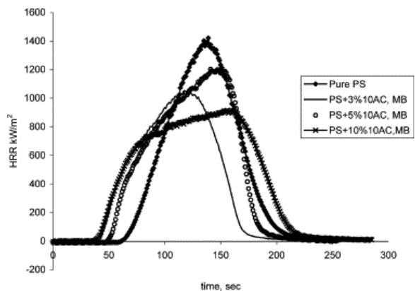
Fig. 16. HRR curves for PS + 10AC clay nanocomposites, melt blending.
