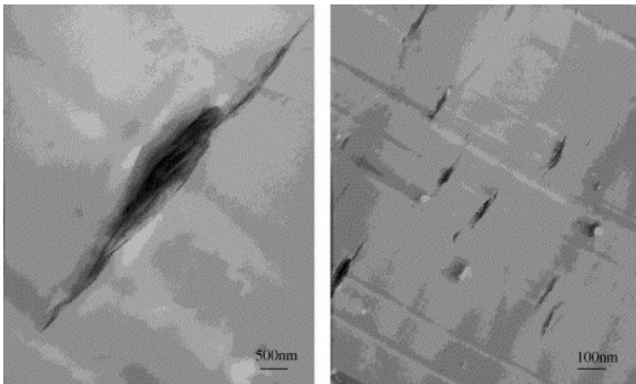
Fig. 7. TEM images for melt blended polystyrene with 3% 10AC clay.
