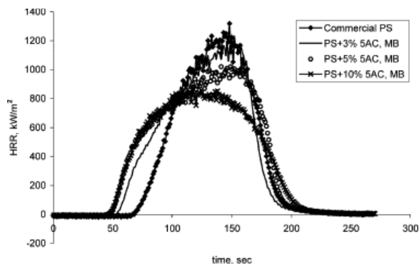
Fig. 14. HRR curves for PS + 5AC clay nanocomposites, melt blending.
