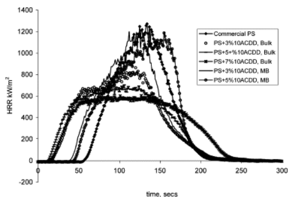
Fig. 17. HRR curves for PS + 10ACDD clay nanocomposites, bulk and melt blending.
