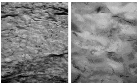
Fig. 8. TEM images for bulk polymerized styrene with 3% 10ACDD clay.
