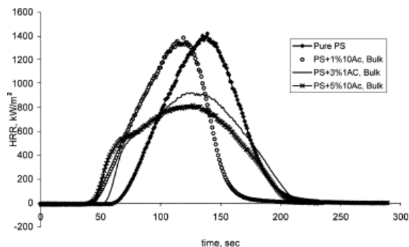
Fig. 15. HRR curves for PS + 10AC clay nanocomposites, bulk.
