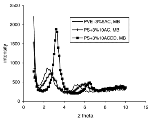
Fig. 3. XRD for PS + clay nanocomposites prepared by melt blending.
