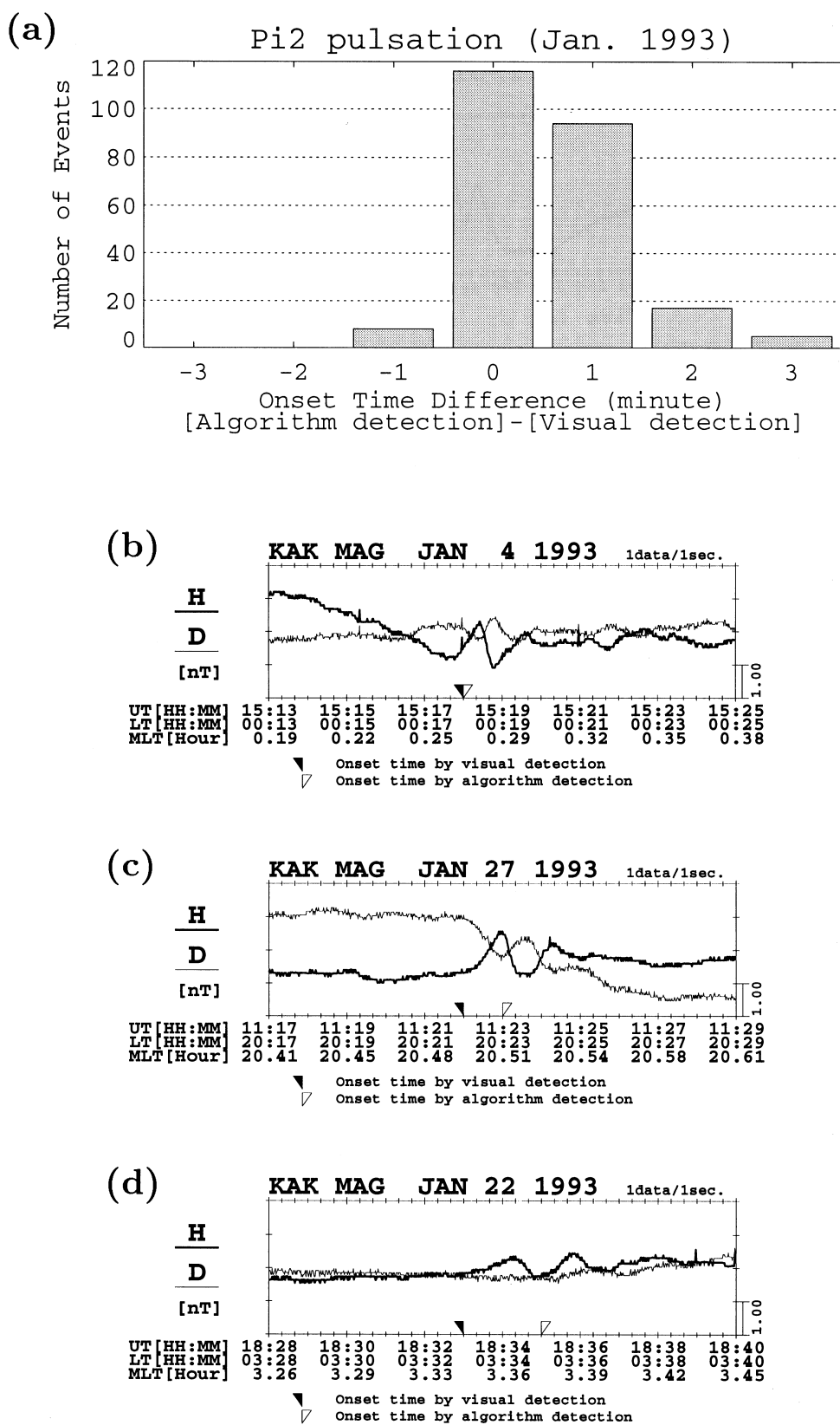
Fig. 4. (a) Distribution of the onset time difference, which is defined as the onset time determined by the algorithm detection minus that by the visual detection. (b)–(d) Examples of Pi 2 pulsations with onset time differences of 0, 1, and 2 minute(s), respectively.
