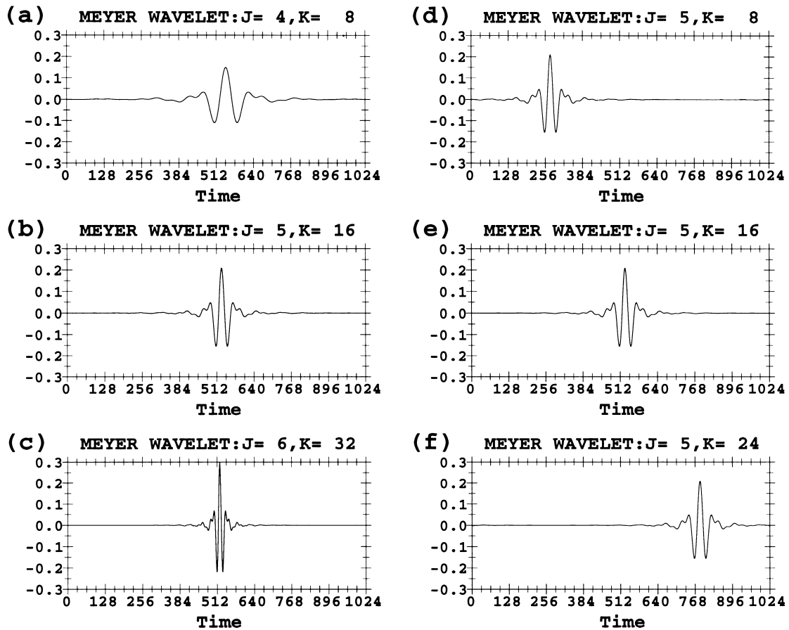
Fig. 1. Time plots of wavelet functions, which were generated from the Meyer wavelet, with (j, k) of (a) (4, 8), (b) (5, 16), (c) (6, 32), (d) (5, 8), (e) (5, 16), and (f) (5, 24).
