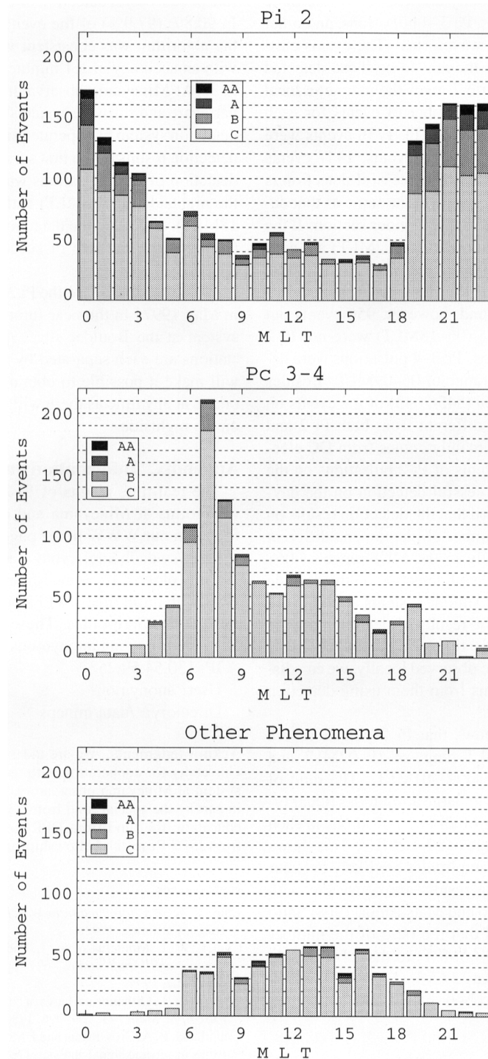
Fig. 7. MLT dependence of the number of events detected at Mineyama, which were classified into three categories according to visual inspection of waveforms. (top) Pi 2 pulsations, (middle) Pc 3–4 pulsations, and (bottom) other phenomena.
