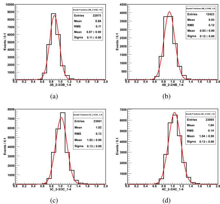
Figure 8. Ratio of the signal in one half to the signal in the other half for two-channel readout PMTs 3B (a), 4B (b), 3C (c) and 4C (d).
