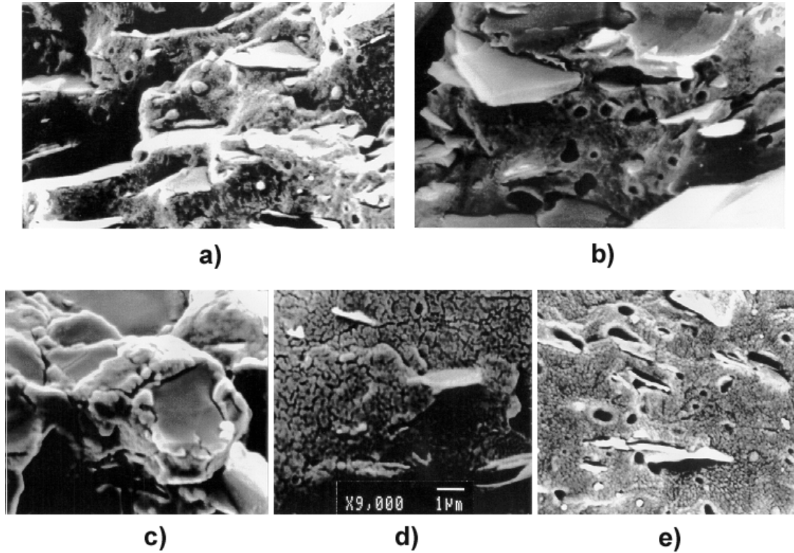
Figure 3: Scanning electron micrographs of hybrid composites; a) surface of unextracted PP with 12 vol.% treated talc and 5 vol.% SEBS, b) surface of xylene extracted PP with 12 vol.% treated talc and 5 vol.% SEBS, c) surface of unextracted PP with 12 vol.% treated talc and 5 vol.% SEBS-gMA, d) surface of xylene extracted PP with 12 vol.% treated talc and 5 vol.% SEBS-gMA, e) surface of xylene extracted PP with 12 vol.% treated talc and 10 vol.% SEBS-gMA
