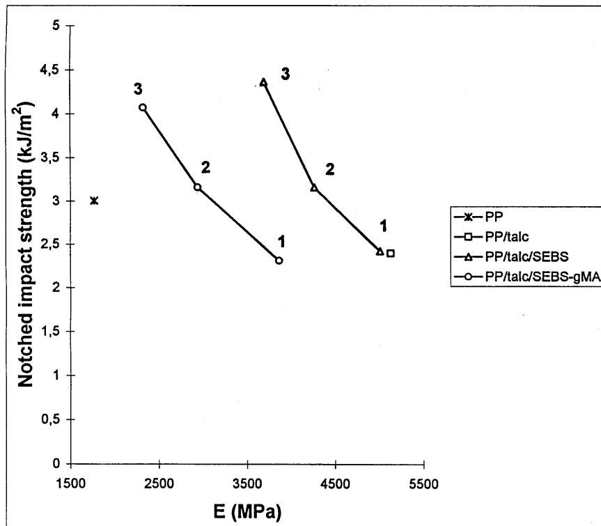
Figure 7: Notched impact strength correlated with Young's modulus for PP hybrid composites with 12 vol.% talc and with 2.5 vol.% (1), 5 vol.% (2) and 10 vol.% (3) elastomer
