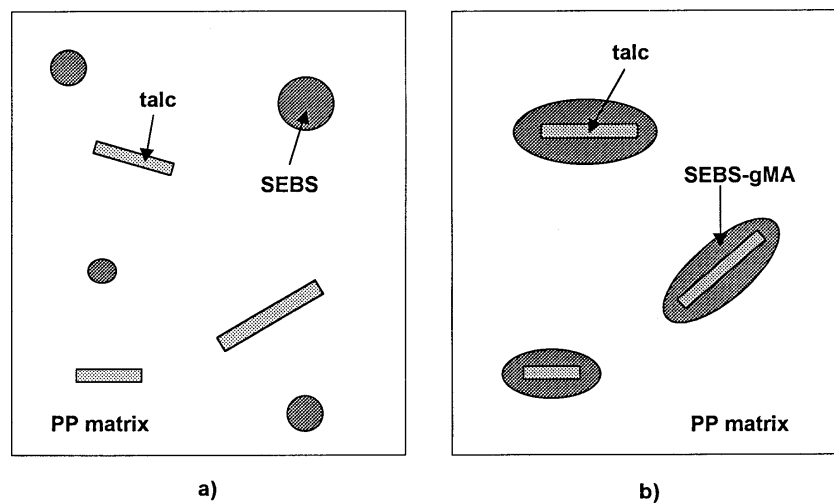
Figure 2: Morphologies of PP hybrid composites: a) three phase morphology with separately dispersed elastomer and filler particles b) two phase morphology with core-shell particles (filler particle core and elastomeric shell)
