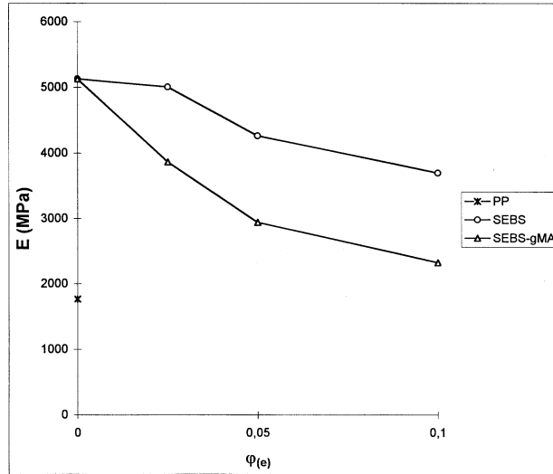
Figure 1: Young's modulus of pure PP and modified PP/treated talc composites as a function of elastomer volume fraction at talc content 12 vol.%
