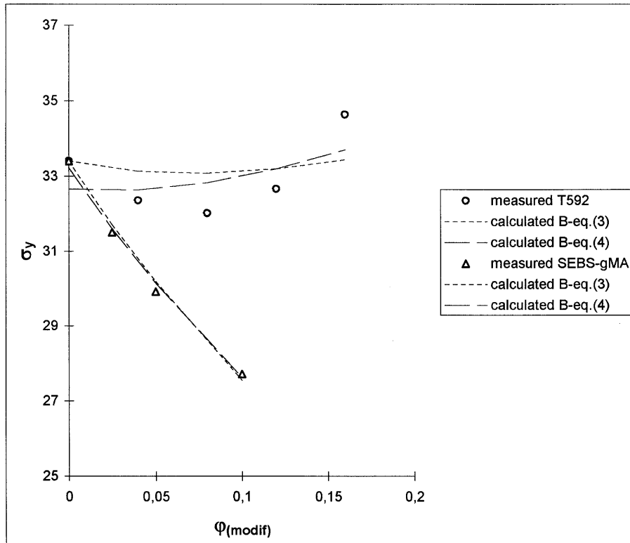
Figure 6: Comparison of calculated and measured values of yield stress for PP/T592 and PP/SEBS-gMA systems as a function of modifier (talc or elastomer) volume fraction
