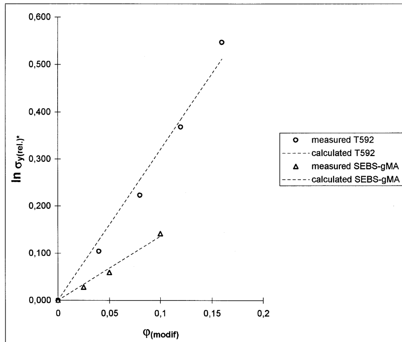
Figure 4: Dependence of linearized yield stress according to equation (2) as a function of modifier volume fraction
