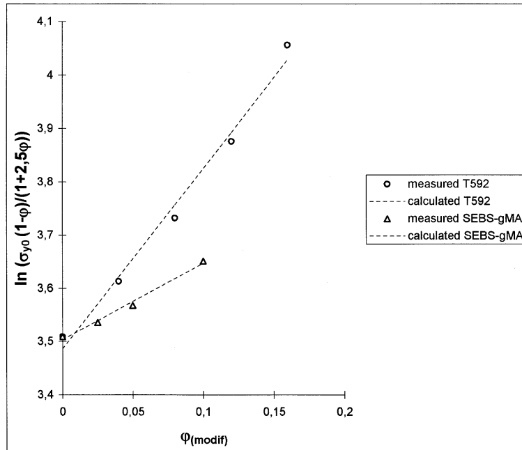
Figure 5: Dependence of linearized yield stress according to equation (3) as a function of modifier volum fraction
