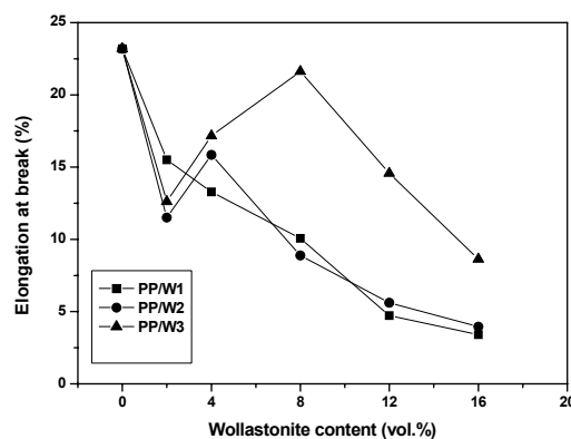
Figure 5. Elongation at break of the PP/wollastonite composites in dependence of wollastonite content.
