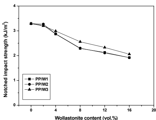
Figure 6. Notched impact strength of the PP/wollastonite composites in dependence of wollastonite content.
