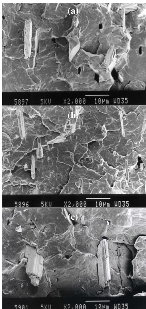
Figure 1. SEM micrographs of fractured samples of the PP/wollastonite (96/4 vol.%) composites a) PP/W1, b) PP/W2 and c) PP/W3.
