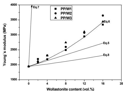
Figure 2. Comparison of experimental data with theoretical predictions of Young's modulus for the PP/wollastonite composites in dependence of wollastonite content.
