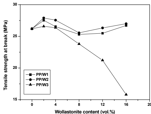
Figure 4. Tensile strength at break of the PP/wollastonite composites in dependence of wollastonite content.
