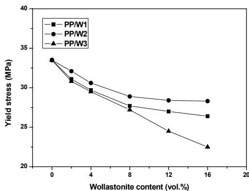
Figure 3. Yield stress of the PP/wollastonite composites in dependence of wollastonite content.
