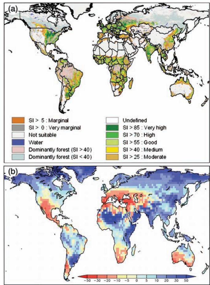
Figure 5.1. (a) Current suitability for rain-fed crops (excluding forest ecosystems) after Fischer et al., 2002b). SI = suitability index; (b) Ensemble mean percentage change of annual mean runoff between present (1981 to 2000) and 2100 (Nohara et al., 2006).
