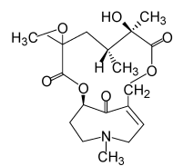
Petasitenine
