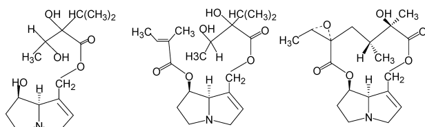
Intermedine
