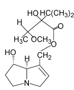
Heliotrine
