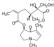
Hydroxysenkirkine
