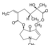
Senkirkine
