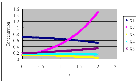
Figure 2. Expanded time profile with spline.
