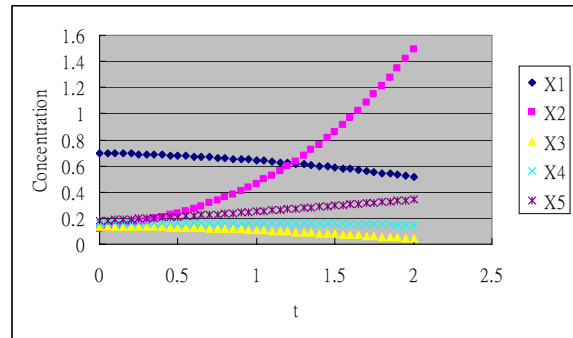
Figure 1. Basic time profile of five genes
