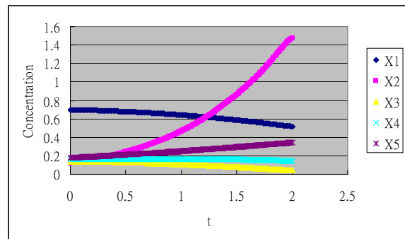
Figure 3. Expanded time profile with ANN.
