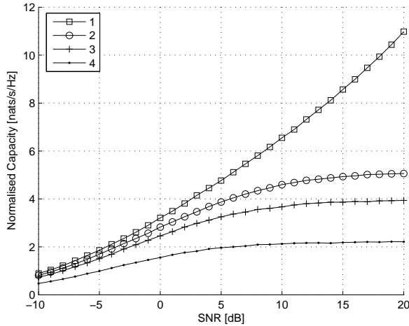
Fig. 4. Capacity lower bound for the 4 \times 4 \times 4 Relay MIMO system ( S \rightarrow R \rightarrow D ) with Spatial Correlation at the transmitter only with d_t/\lambda_c = 0.1 1. Error free system - Variance of error \sigma_e^2 = 0.0 2. Variance of error \sigma_e^2 = 0.1 3. Variance of error \sigma_e^2 = 0.2 4. Variance of error \sigma_e^2 = 0.5
