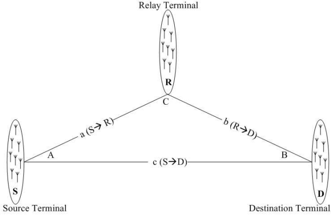
Fig. 1. Schematic representation of the Relay MIMO channel. MIMO antenna systems are placed in the corners of the triangle as shown in [4] and [6].
