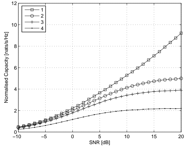
Fig. 3. Capacity lower bound for the 4 \times 4 direct path MIMO system ( S \rightarrow D ) with Spatial Correlation at the transmitter with d_t/\lambda_c = 0.1
