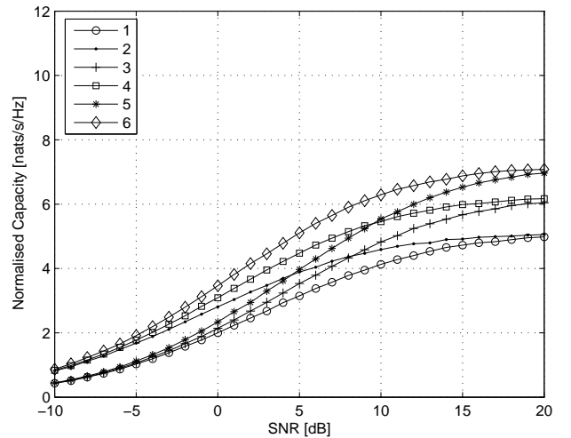
Fig. 5. Capacity lower bound for the direct path 4 \times 4 MIMO system ( S \rightarrow D ) versus the 4 \times 4 \times 4 Relay MIMO system ( S \rightarrow R \rightarrow D ) with Spatial Correlation at the transmitter and Variance of error \sigma_e^2 = 0.1 .
