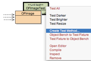
Fig. 2. A reference class and attached test class. The test class is marked with a stereotype and different colour. A context menu shows the test class operations.
