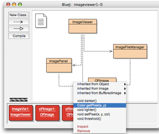
Fig. 1. The main interface of BlueJ. The window includes a class diagram, and interactively created objects on the object bench at the bottom. Both classes and objects have context menus for interaction.
