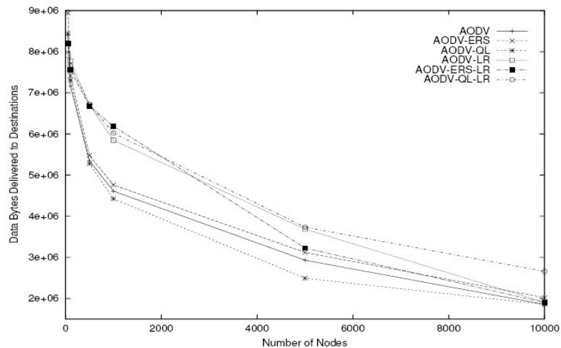
Figure 6: AODV scalability in terms of delivery success (Lee et al., 2003)
