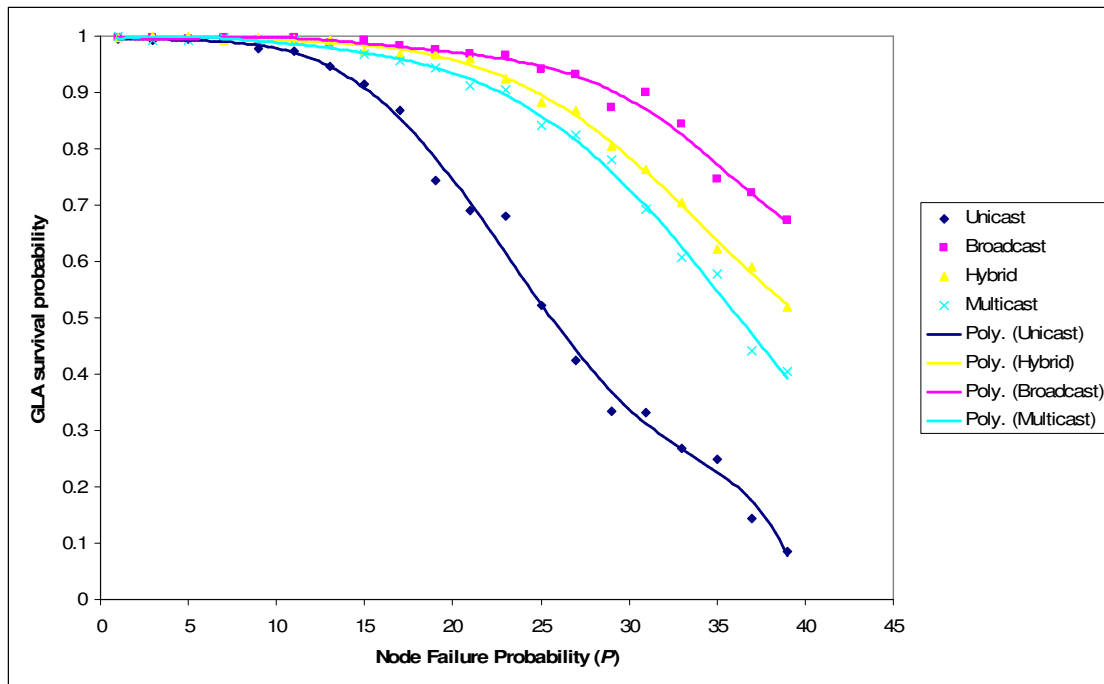
Figure 29: Failure tolerance
