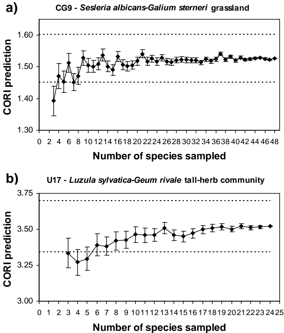
Figure 2. Sensitivity analysis illustrating how the CORI prediction varies with increasing sample size in two communities of contrasting species richness, where (a) n=48 species and (b) n=24 species. Bars show \pm one standard error. Dotted horizontal lines show limits of \pm 5\% from CORI value calculated using all available species (Jones et al. 2007).
