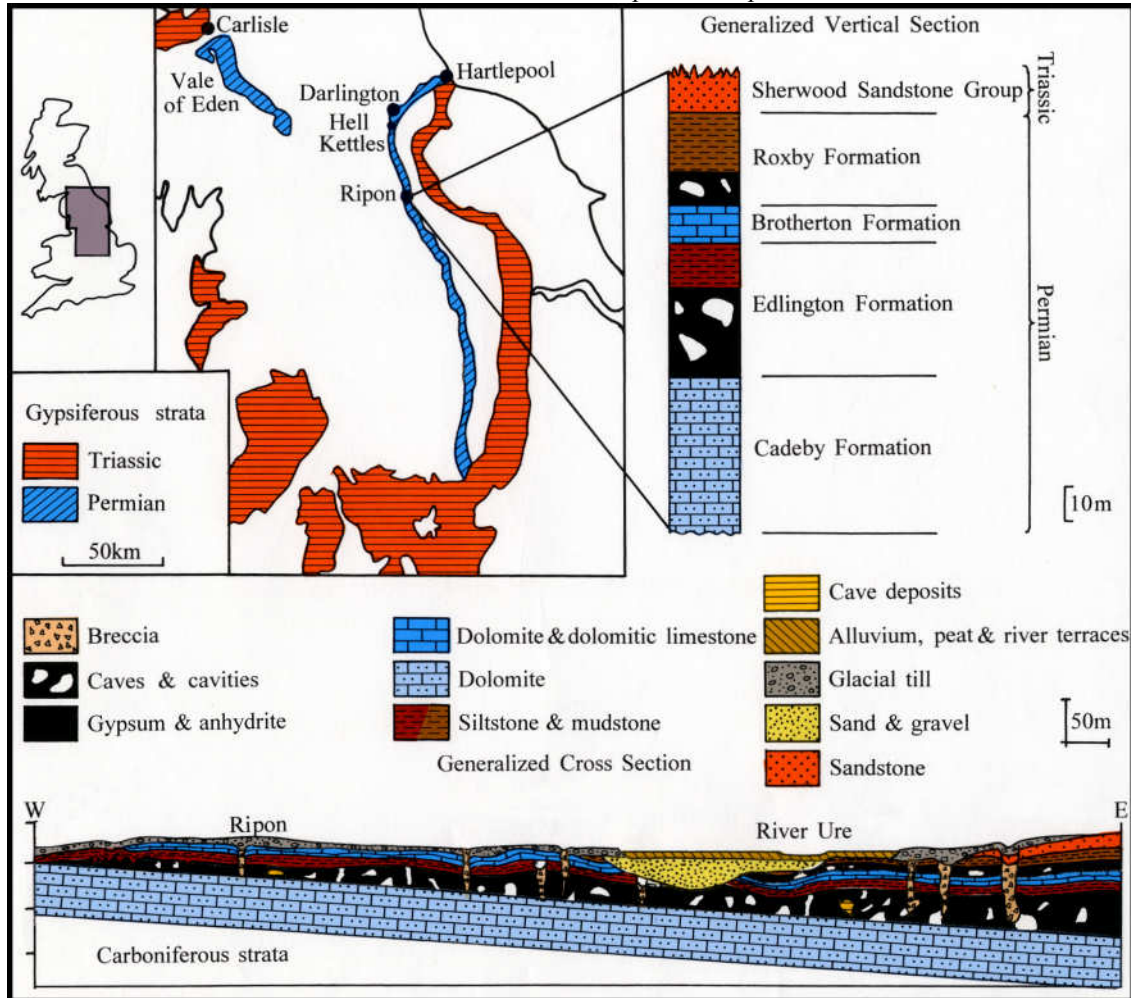
Figure 3. Regional geology of the Permian and Triassic gypsiferous sequences with a cross-section from west to east through the Ripon area showing the easterly dipping dolomite and gypsum sequence cut into by the glacial valley of the River Ure. The key on this figure is also the key to figures 7 and 8.
