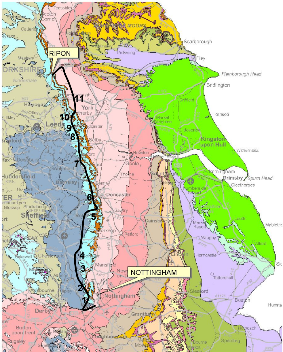
Geology, extracted from the British Geological Survey 1:625,000 scale bedrock geology map (not to scale)
