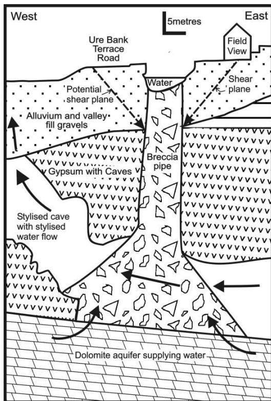
Figure 11. Schematic cross section and photograph of the Ure Bank Terrace collapse in early May 1997.
