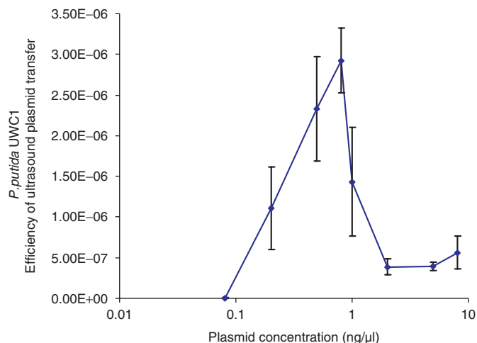
Figure 6. The effect of plasmid concentration on UDD of P. putida UWC1. High concentration plasmid reduced UDD efficiency ( P < 0.05 ).
