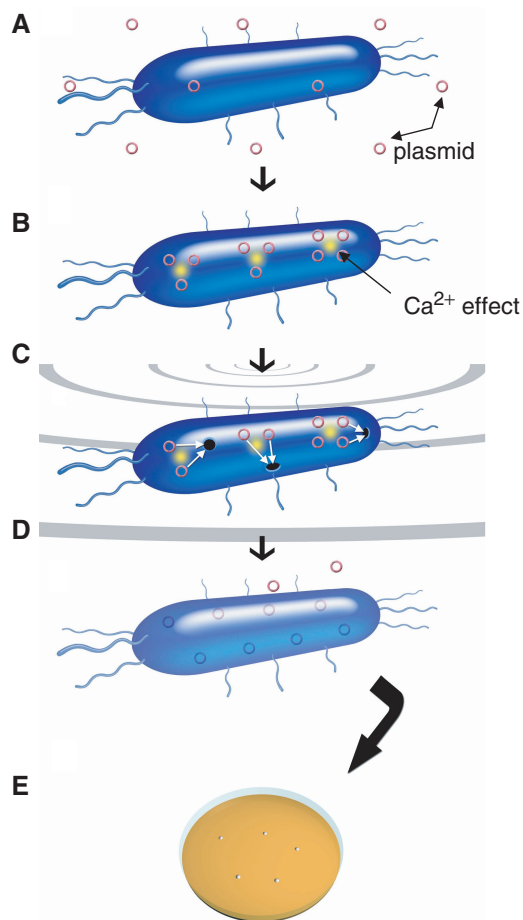
Figure 4. Illustration of proposed mechanism of ultrasound DNA transfer. (A) A bacterial cell and plasmid DNA are suspended in an aqueous solution. (B) 50 mM \text{CaCl}_2 promotes transformation. (C) Ultrasound generates pores in cell membranes through which plasmids enter the cell. (D) Pores are closed and plasmids are retained in the cell. (E) Bacteria acquire new functions after taking up plasmid DNA.
