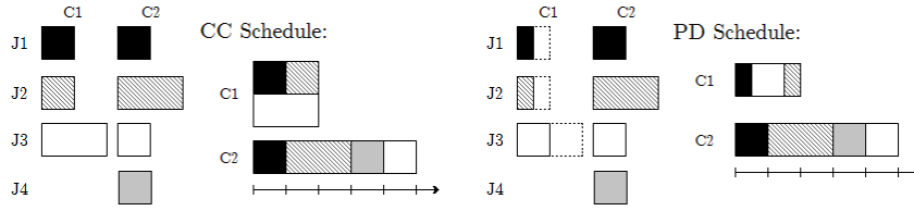
■ Figure 3 An instance I of CC \parallel \sum w_j C_j , and its image I' = TSPT(I) . The schedules were constructed with List-LPT using the same permutation for I and I' .
