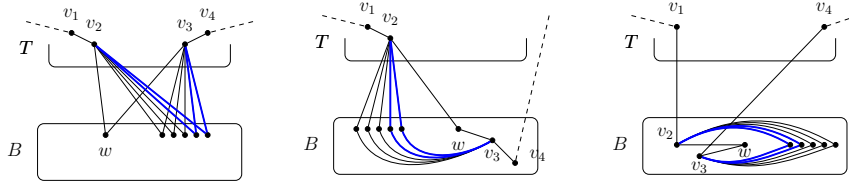
■ Figure 4 Cases 1–3 in Proposition 4.4.
