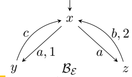
Figure 1 A Büchi automaton.
