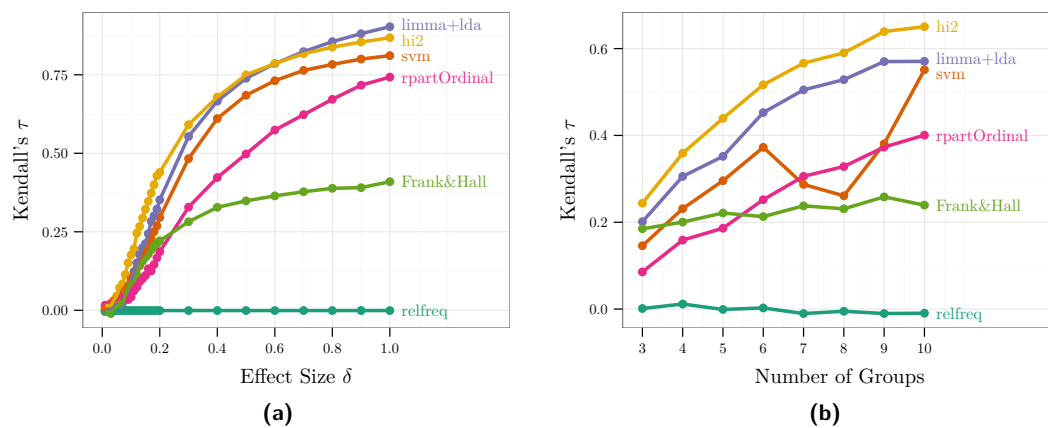
■ Figure 1 This Figure presents the results from a simulation study. Gene expression of 1000 genes was simulated for 90 patients belonging to 5 ordinal classes. 60 patients were used to train the classifiers and the remaining 30 patients formed the test set. Shown is Kendall's \tau comparing the classification result (the predicted class) with the true value. Kendall's \tau takes values between -1 (perfect negative correlation) and 1 (perfect correlation). The left panel (a) shows the results for different effect sizes \delta . 50 genes have been simulated to be differentially expressed across the 5 ordinal classes and \delta is the level of differential expression. The right panel (b) shows results for a fixed effect \delta = 0.2 but different number of groups.
