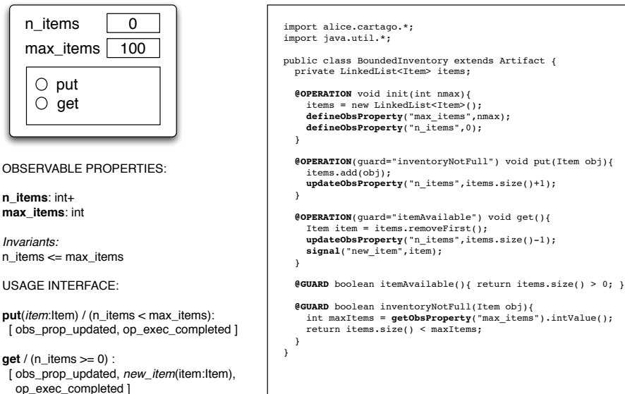
Fig. 2. A simple bounded-inventory artifact, exploiting operation control guards to synchronize agent use of the inventory.
