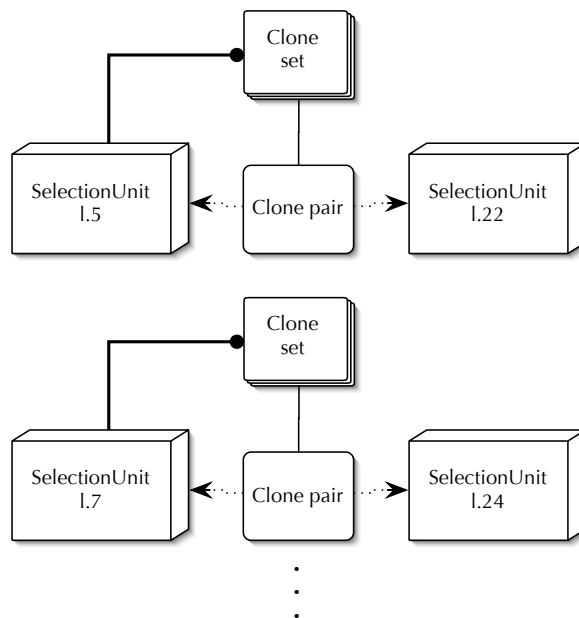
Figure 2: Example: lines as selection units
