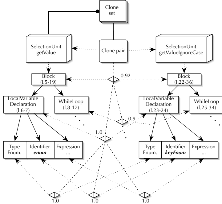
Figure 4: Example: AST subtrees as comparison units
