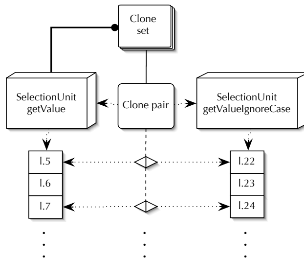
Figure 3: Example: lines as comparison units
