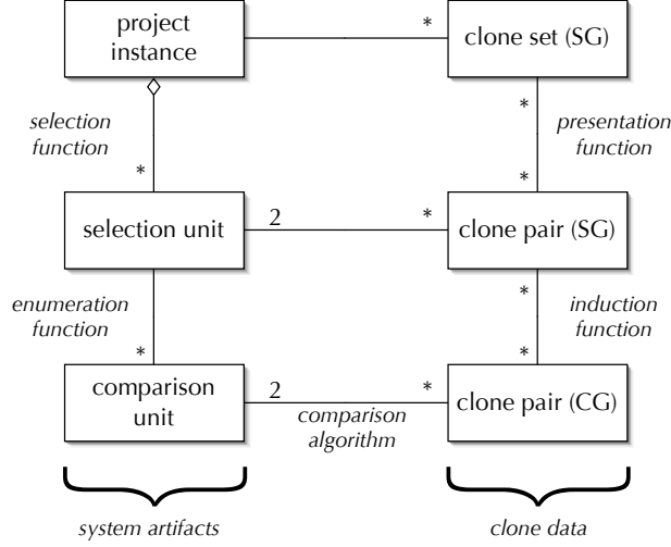
Figure 5: Overview of the generic clone model
