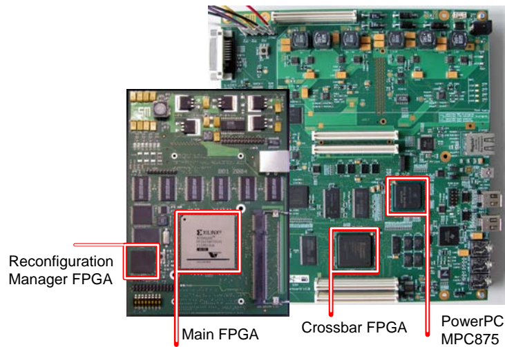
Fig. 6. ESM: BabyBoard and MotherBoard. The BabyBoard is mounted on the application-specific MotherBoard, in this case a multimedia board, using 4 connectors.
