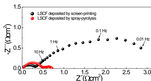
Figure: Impedance spectra of LSCF cathodes deposited by spray-pyrolysis and conventional screen-printing on BCZY electrolytes.
