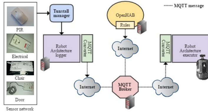
Fig. 1. Framework overview.
