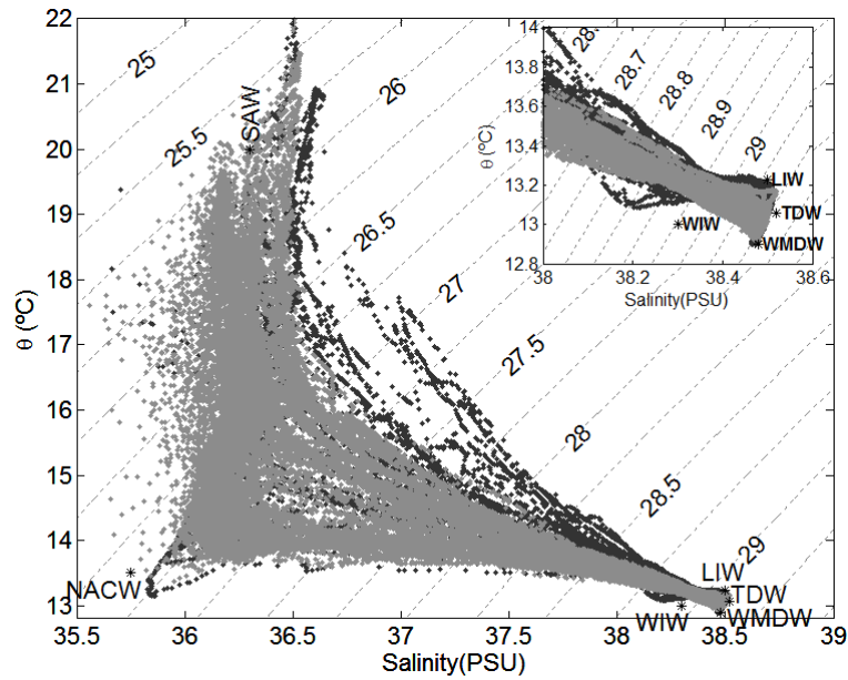
Figure 2. \theta -S diagram of the whole data set ( GIC data in grey, INGRES data in black). The locations of the water masses defined by the thermohaline properties showed in Table 1 are marked by stars, with their acronyms aside. The inset is a zoom of the Mediterranean Water zone of the diagram.
