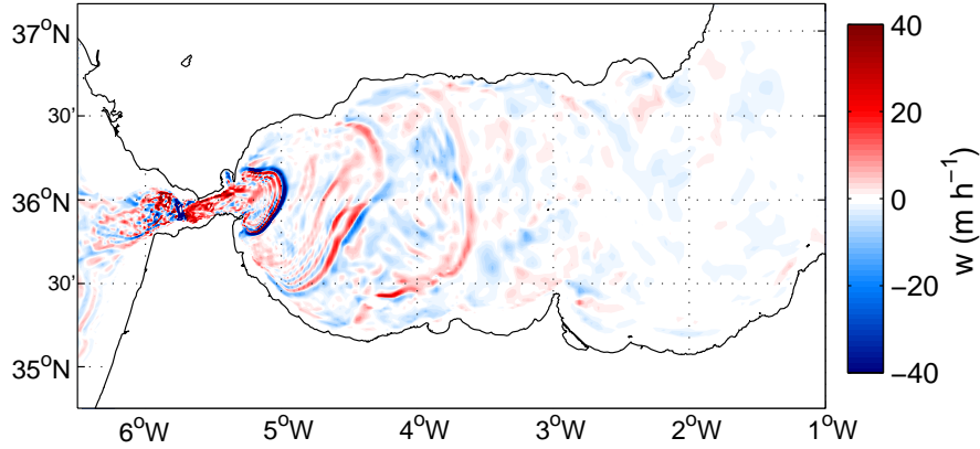
Figure 11. a) Synoptic field of vertical velocity at z = -88.5\text{m} , as simulated in the TID experiment.
