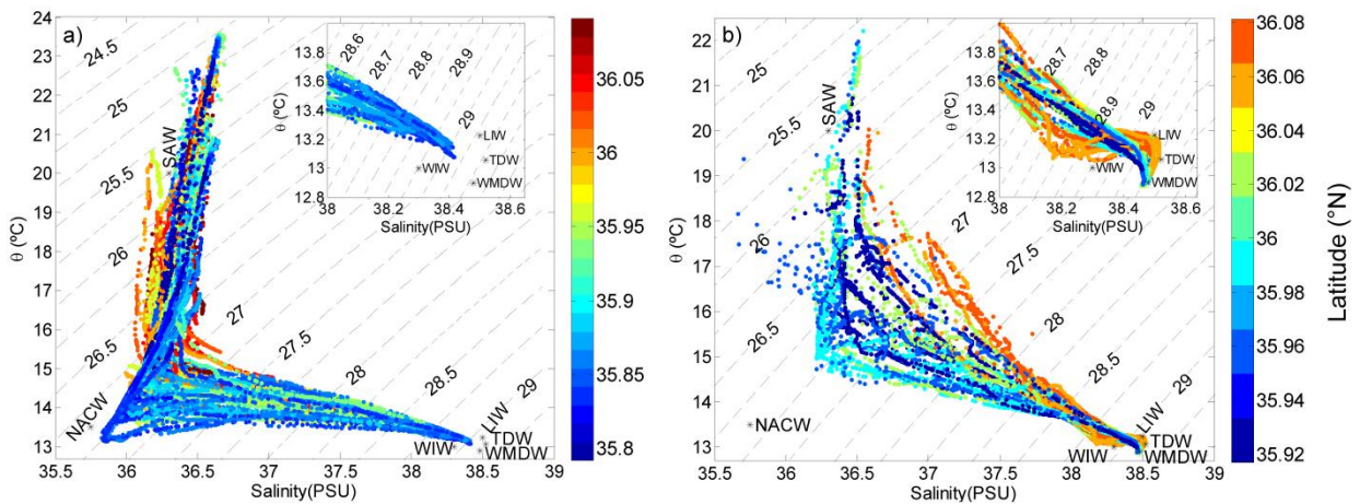
Figure 6. \theta - S diagram showing the CTD data collected at TES (a) and TAC (b) transects during the INGRES project from 2004 up to the present. The colour scale indicates latitude and the contour lines shows \sigma_{\theta} . Black stars mark the \theta - S pairs of the water masses involved in the exchange (see Table 2). The insets zoom in the Mediterranean water zone of the diagram.
