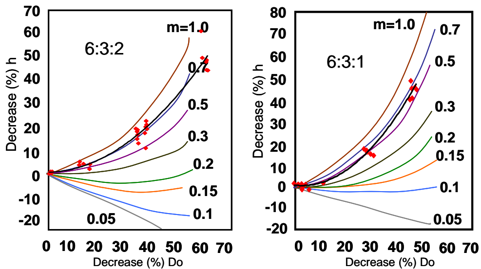
Figure 6. Curves Ring Compression Test and experimental curve
