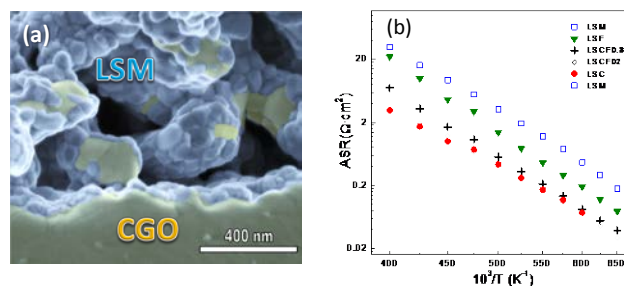
Fig. 1. (a) SEM of LSM cathode deposited by spray-pyrolysis on a porous CGO backbone and (b) area specific polarization resistance (ASR) values for different cathodes.
