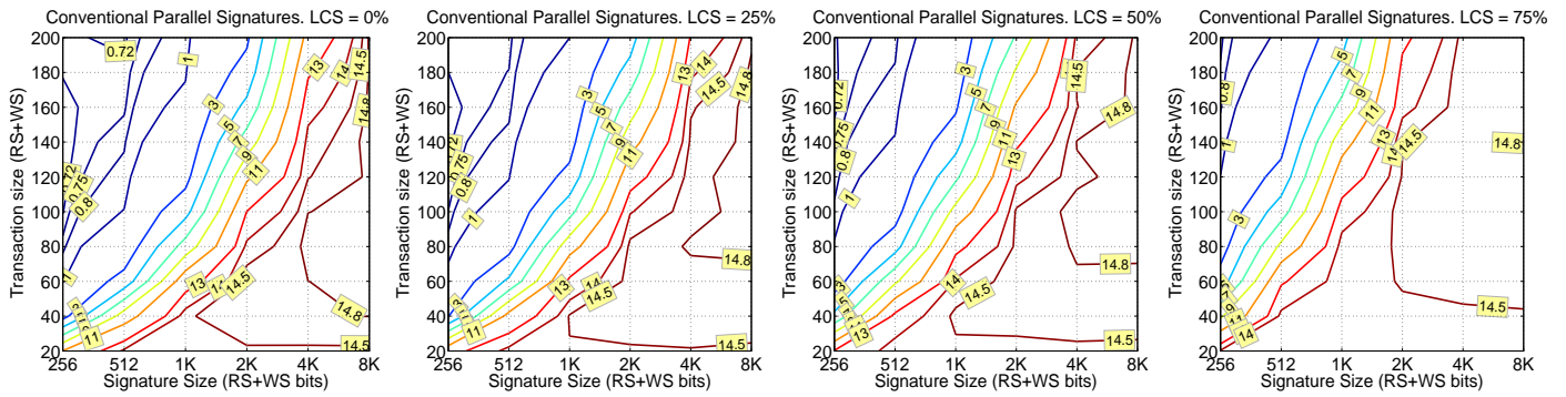
Fig. 5: Iso-speedup contour plots of conventional parallel signatures with lcs ranging from 0% (left) to 75% (right).
