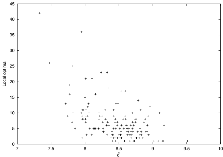
Fig. 4 Number of local optima against the autocorrelation length \ell for instances with n = 20 .
