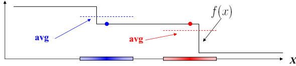
Fig. 2 In plateaus the average-based selection strategy could distinguish between two solutions with the same fitness value.
