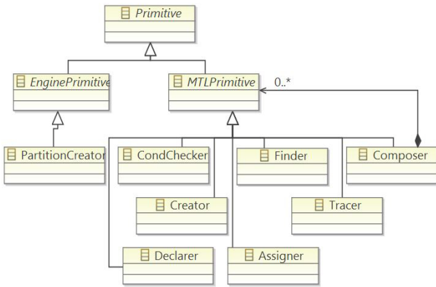
Figure 1: Primitives Class Diagram.
