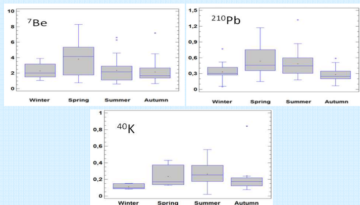
Fig. 1.-Seasonal variation of specific activities of 7 Be and 210 Pb
