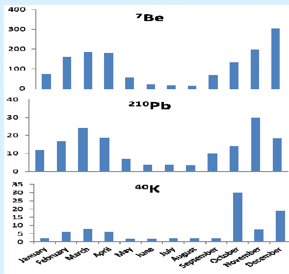
Fig.2. Depositional fluxes of Be-7 and Pb-210 during the sampling period: January 2005-December 2012.
