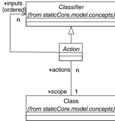
Figura 2.3: Paquete actions.model.concepts.
