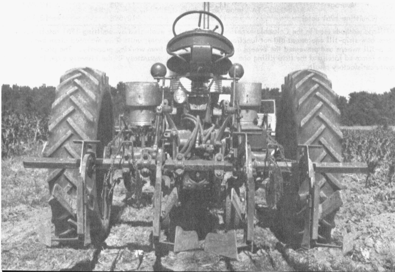
Fig. 6 A tractor equipped to plow the middles with rear-mounted "half plows" at the time of the first cultivation. Regular front sweeps set to work close to the row may be used for more complete weed control, if needed. Also, fertilizer may be applied as desired.
