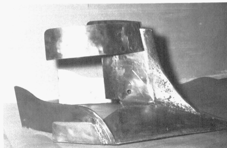
Fig. 2 The basic strip plow unit which was developed from these studies. The top wings force the surface soil and trash outward, and the lower wings move moist, trash-free soil in the bottom of the furrow slice toward the center of the strip.
