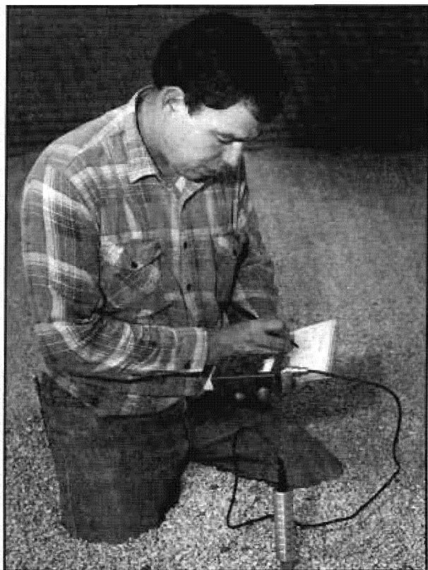
Figure 5. Monitoring and recording grain temperature with an electronic thermometer. You should probe several areas inside the bin for hot spots.
