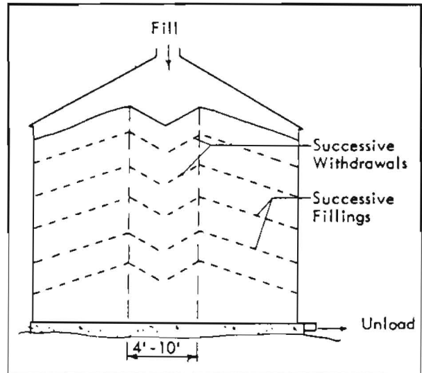
Figure 7. Withdrawing grain during filling removes many fines and helps prevent mold growth.
