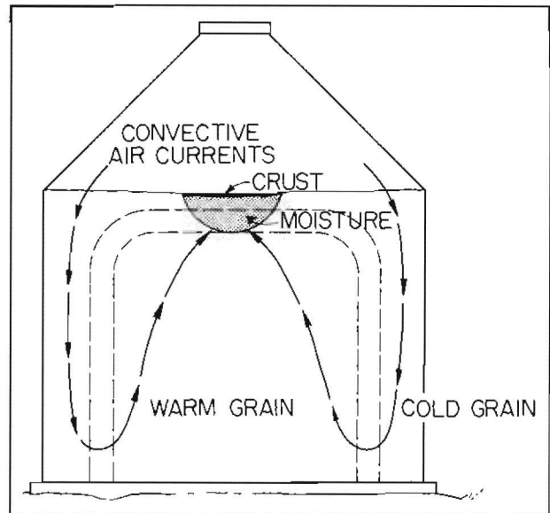
Figure 1. How grain temperatures cause moisture migration.
