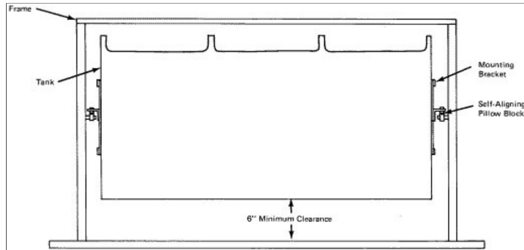
Figure 5 Mounting frame for tank.
