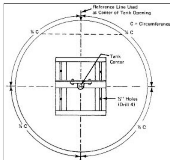
Figure 4 Measuring detail for locating center.
