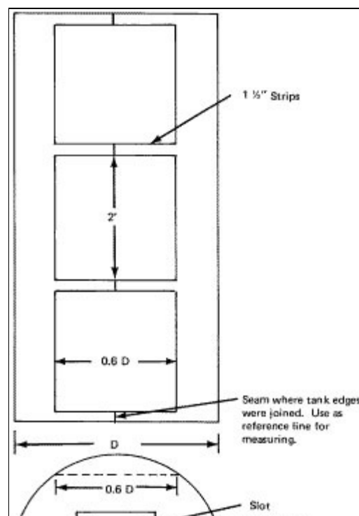
Figure 2 Detail on tank discharge opening.
