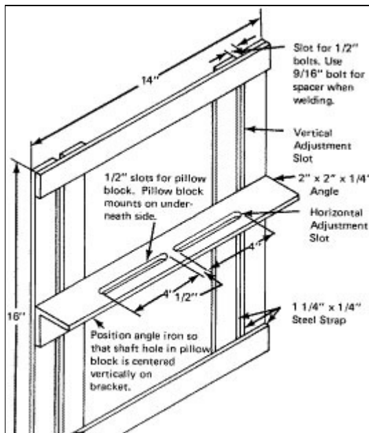
Figure 3 Detail on end bracket.
