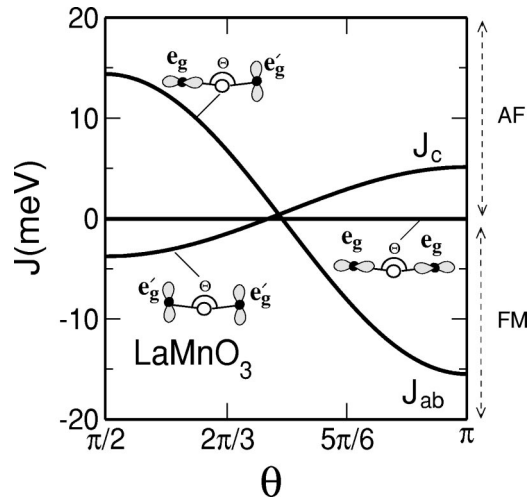
FIG. 10. Exchange interaction in \text{LaMnO}_3 with the full Hamiltonian, i.e., with J_H = 1 eV and with t_{2g} hopping included. The intraplane and interplane exchanges, J_{ab} and J_c , correspond to the e_g - e'_g and e'_g - e'_g orbital orientations, respectively.
