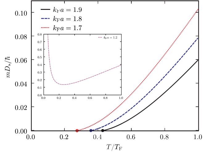
FIG. 3 (color online). Panel (a): spin diffusion constant D_s as a function of temperature T for various interaction strengths k_F a > \pi/2 . Panel (b): spin diffusion constant for k_F a = 1.2 < \pi/2 .
