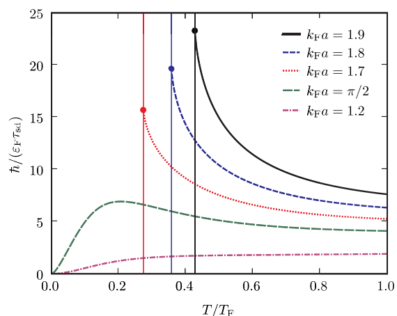
FIG. 1 (color online). Spin drag relaxation rate 1/\tau_{sd}(T) as a function of temperature T , for various values of the interaction parameter k_F a . The Fermi energy is denoted by \varepsilon_F = k_B T_F = \hbar^2 k_F^2 / 2m . Note that for k_F a > \pi/2 , the spin drag relaxation rate shows a distinctive upturn when the critical temperatures, indicated by thin vertical lines, are approached from above. In particular, we have T_c \approx 0.43T_F for k_F a = 1.9 , T_c \approx 0.36T_F for k_F a = 1.8 , and T_c \approx 0.27T_F for k_F a = 1.7 . For k_F a < \pi/2 no ferromagnetism occurs within mean-field theory. In that case 1/\tau_{sd}(T) is smooth throughout the temperature range and exhibits the standard Fermi-liquid behavior 1/\tau_{sd}(T) \propto T^2 for T \rightarrow 0 .
