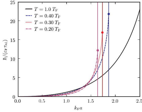
FIG. 2 (color online). Spin drag relaxation rate 1/\tau_{sd} as a function of k_F a for various temperatures. The thin vertical lines indicate the critical values of the interaction parameter k_F a at which ferromagnetism occurs.
