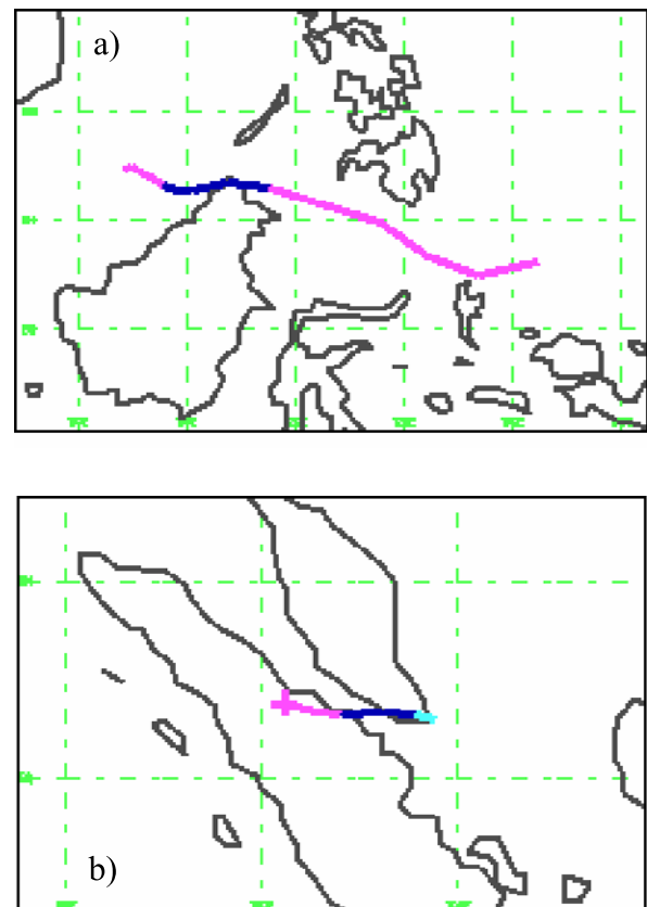
Figure 2. Tracking information for (a) Tropical Storm Greg (24–31 December 1996) and (b) Typhoon Vamei (27–28 December 2001). The mauve, dark blue, and light blue colors indicate a tropical depression, storm, and typhoon, respectively. This figure is adapted from the archive available through the UNISYS website.
