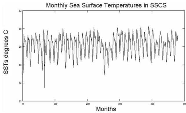
Figure 4. The raw mean monthly SSTs ( ^{\circ}\text{C} ) for the SSCS region from 1963 to 2002.
