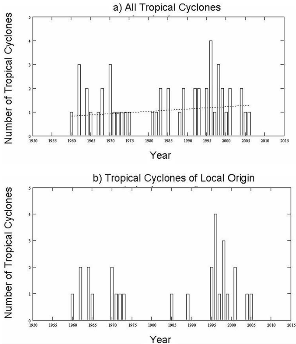
Figure 3. The time series of (a) all tropical cyclones and (b) tropical cyclones of local origin occurring within the SSCS region from 1960 to 2006. In Figure 3a the dashed line is the linear regression line.
