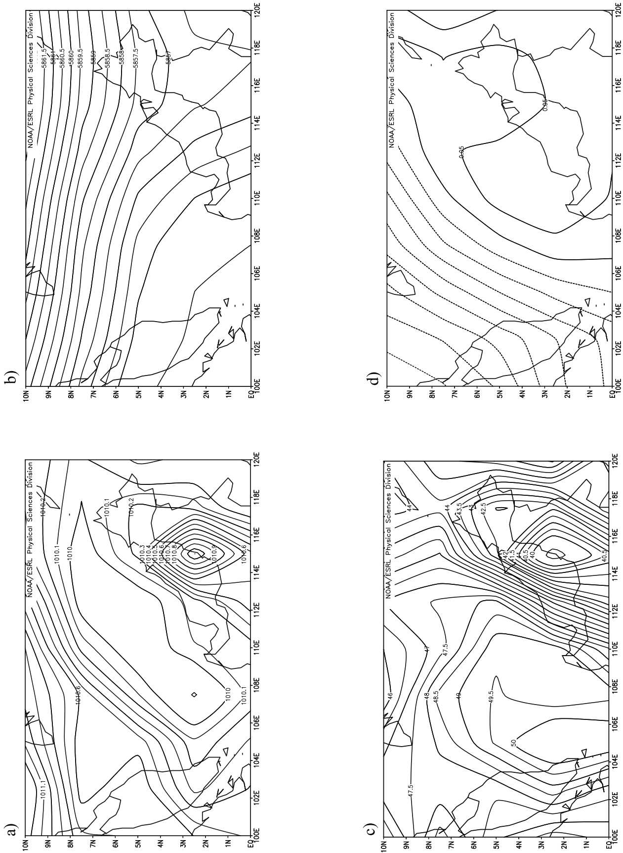
Figure 7. (a–d) As in Figure 6 except for the years in Table 8.
