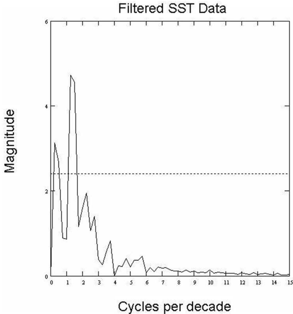
Figure 5. The power spectra for the filtered mean SSTs in the SSCS region. The filter was set in order to remove the signal for time periods smaller than 2 years. The abscissa is cycles per decade; thus 10 is 10 cycles per decade or the annual cycle. The dashed line represents the 99% confidence interval for accepting the red noise spectrum null hypothesis.
