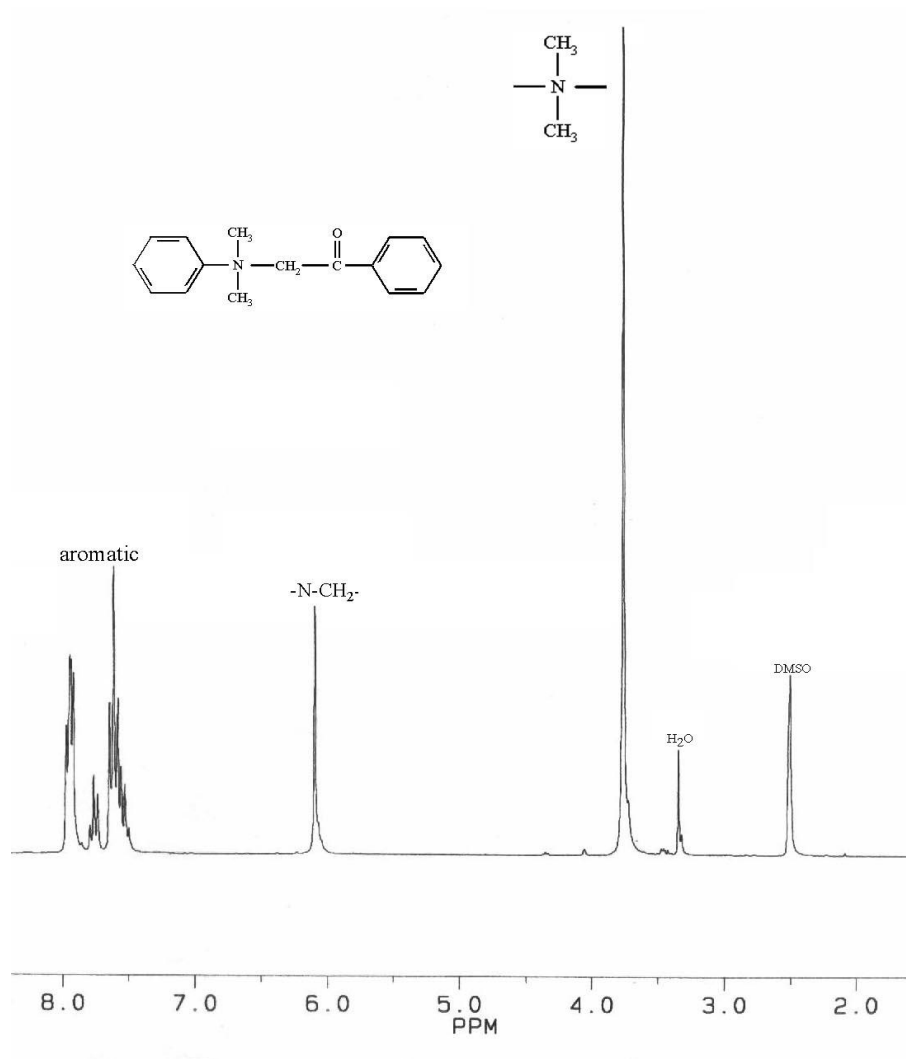
Figure 3.1. ^1\text{H-NMR} spectrum of N -phenacyl N,N -dimethylanilinium hexafluoroantimonate in \text{DMSO}
