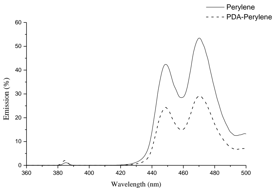
Figure 4.5. Quenching of perylene fluorescence emission at \lambda_{\text{ex}}=386 nm by \text{PDA}^+\text{SbF}_6^- in \text{CH}_2\text{Cl}_2 , [\text{PDA}]=1 \times 10^{-4} mol \text{L}^{-1} , [\text{perylene}]=1 \times 10^{-4} mol \text{L}^{-1}
