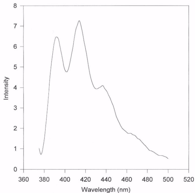
Figure 4.8. Fluorescence spectrum of \text{PDA}^+\text{SbF}_6^- at room temperature.
