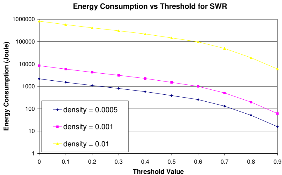
Figure 5.17: Effects of the threshold value and the node densities to the energy consumption in SWR.
