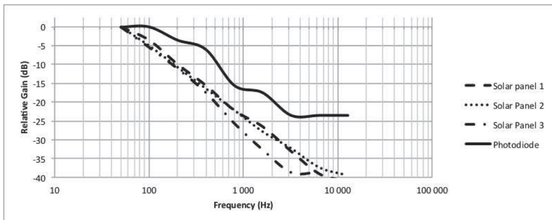
Figure 5: Frequency Response of several optical receiver tested, including solar panels and small footprint photodiodes.
