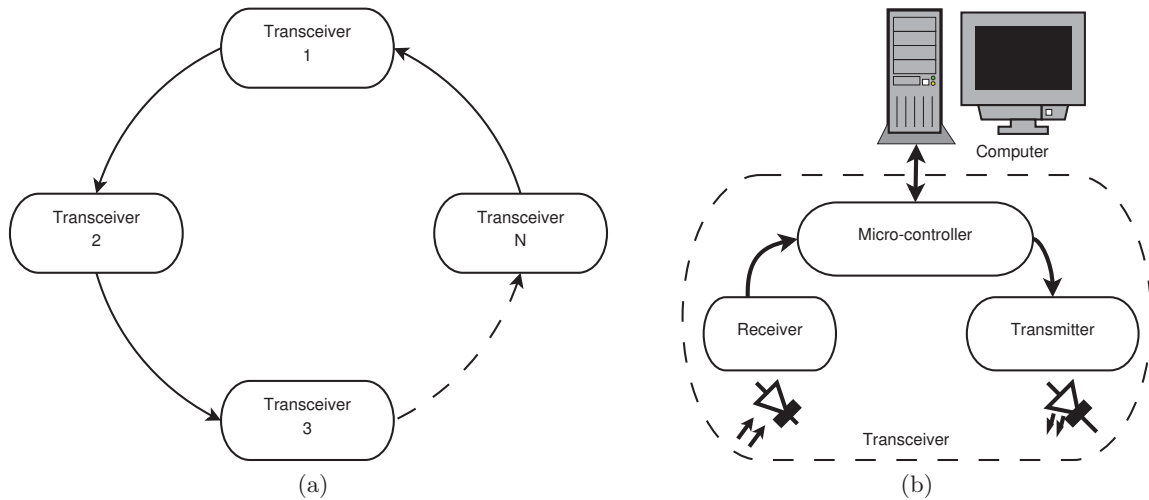
Figure 1: VLC network diagram: (a) Ring configuration; (b) Transceiver diagram.
