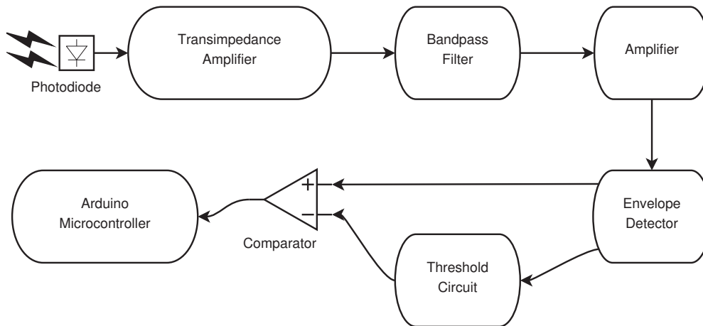
Figure 4: Receiver diagram.
