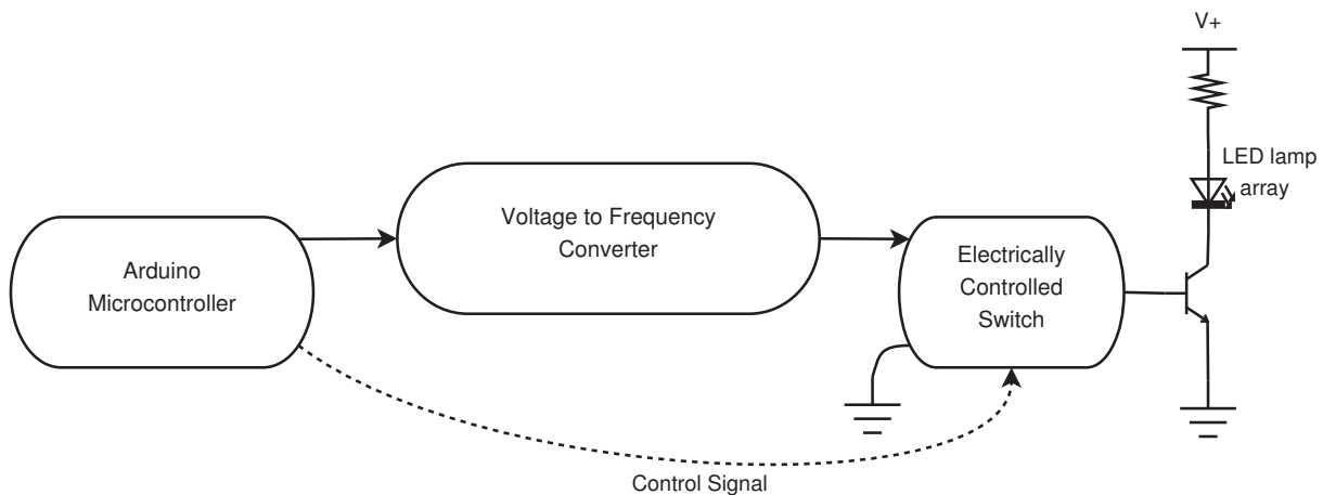
Figure 3: Transmitter diagram.
