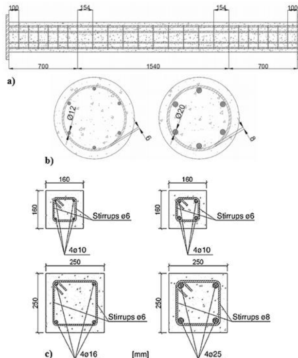
Fig.3 Test specimens
