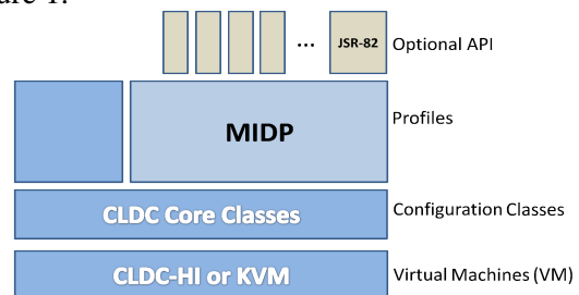
Figure 1 – Client software architecture.
