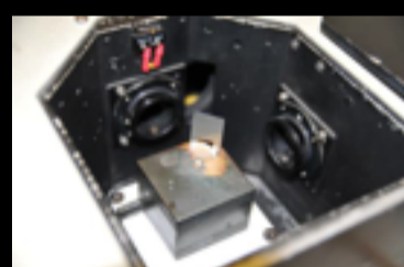
Fig. 2. spectrofluorometer SPEX Fluorolog 212I. Sample ready for lecture.
