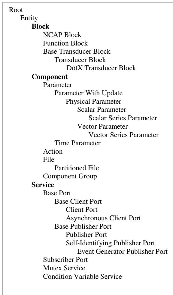
Fig. 2. IEEE 1451.1 Std class hierarchy.
