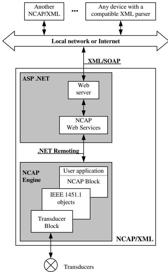
Fig. 6. NCAP/XML architecture.
