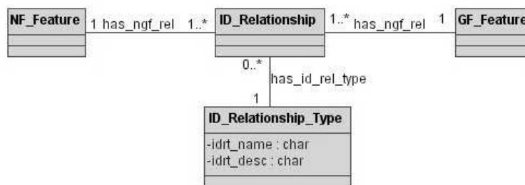
Figure 5. Inter-domain relationships class diagram
