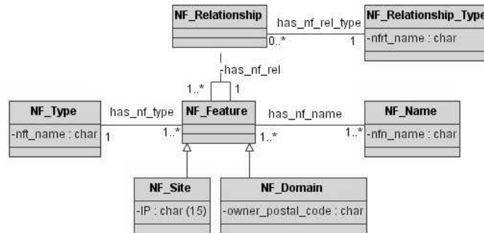
Figure 4. Network domain class diagram
