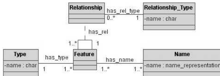
Figure 2. GKB information meta-model
