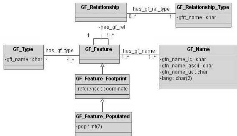
Figure 3. Geographic domain class diagram
