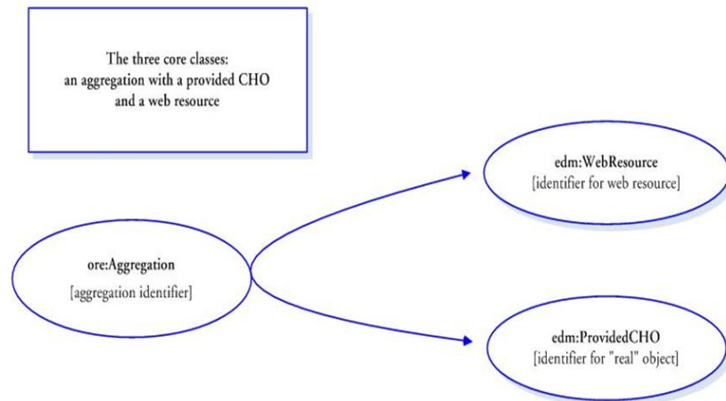
Fig. 1. Basic data model
