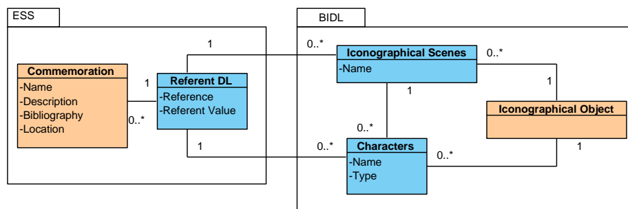
Fig. 4. UML Analysis Class Diagram of the Conceptual Relationship between the ESS and BIDL Entities
