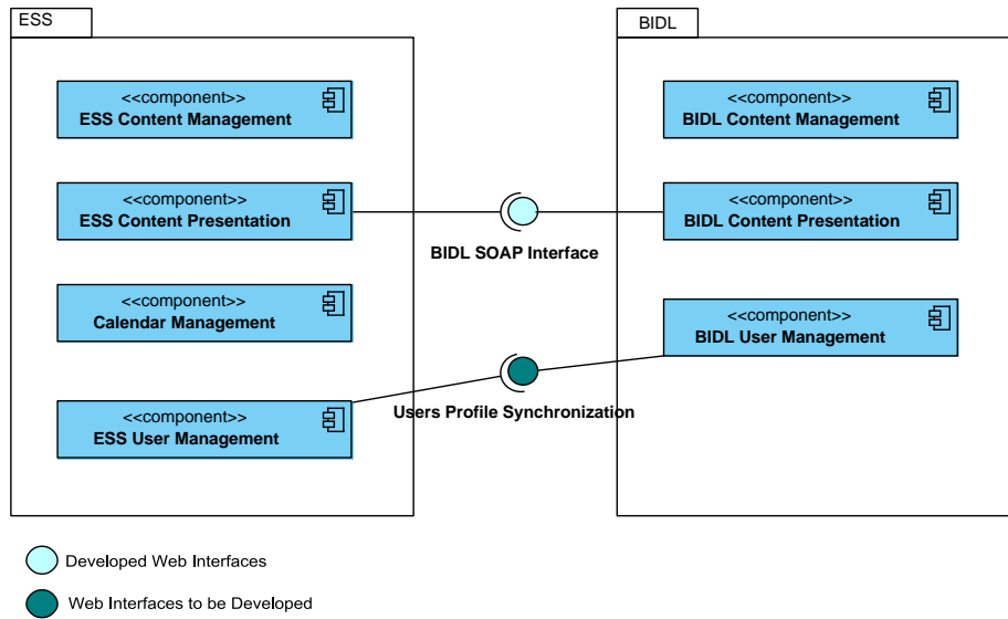
Fig. 5. UML Deployment Diagram of the Web Service Interfaces
