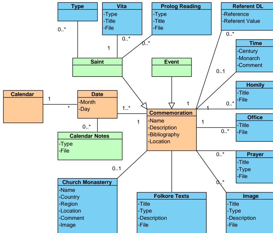
Fig. 3. UML Analysis Class Diagram of the main entity classes in the Encyclopaedia Slavica Sanctorum
