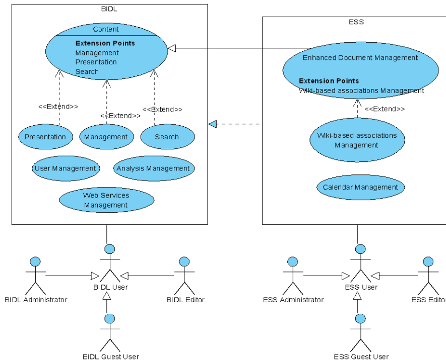
Fig. 2. UML Use Case Diagram
